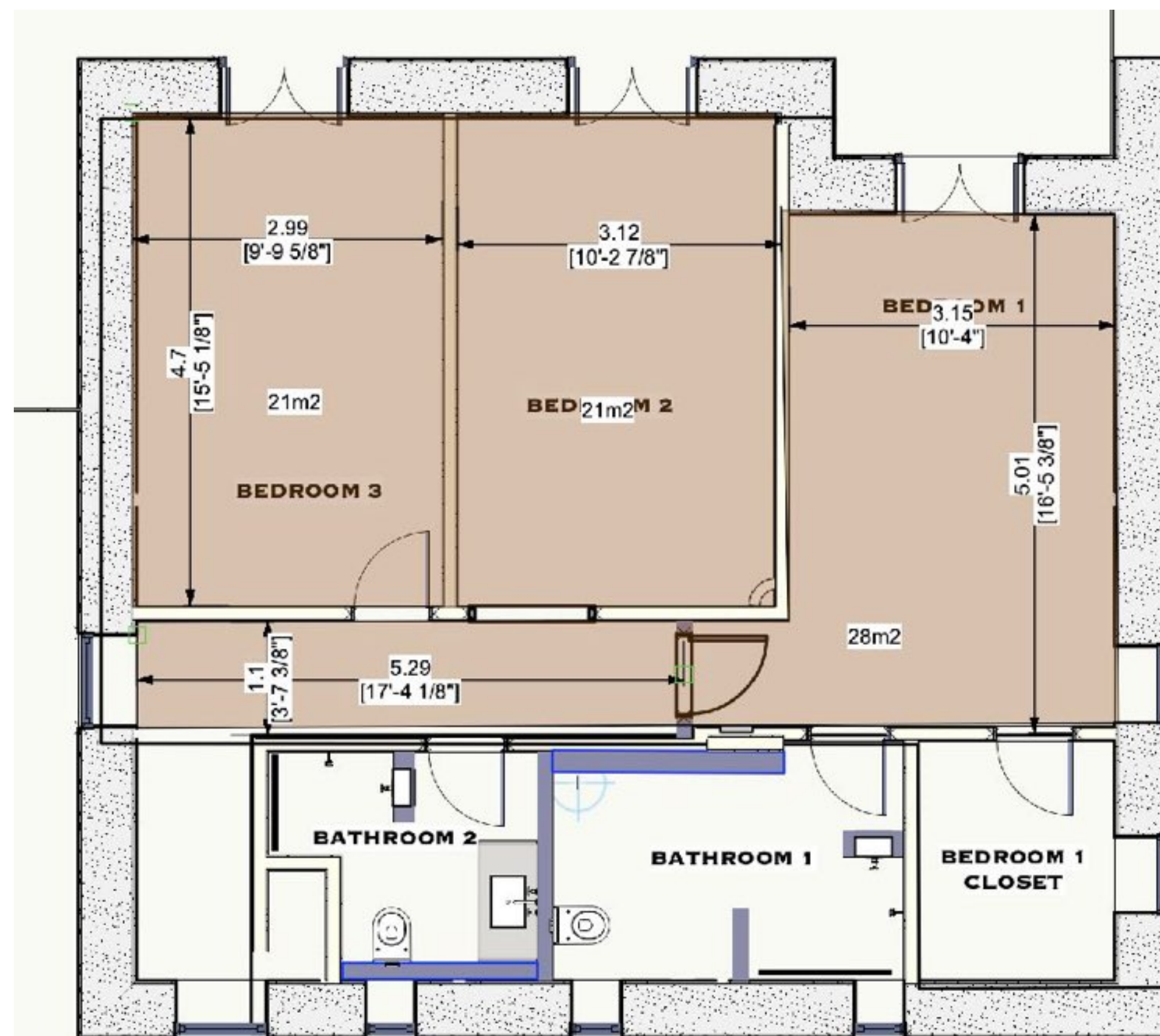
ΕΠΑΝΩ UPSTAIRS 70m 2
